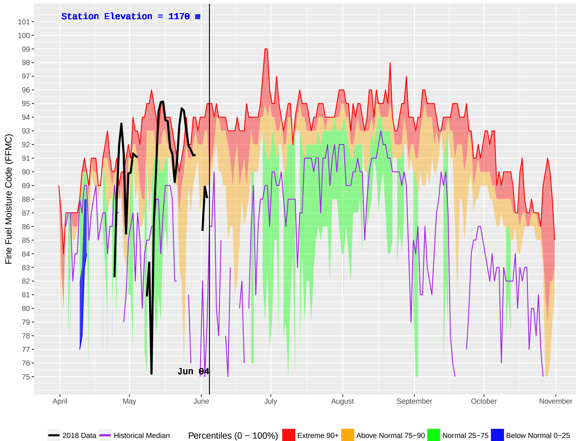
YOUNG LAKE (235) : Historical (2001–2016) and Current (2018) Noon Fine Fuel Moisture Code (FFMC)
