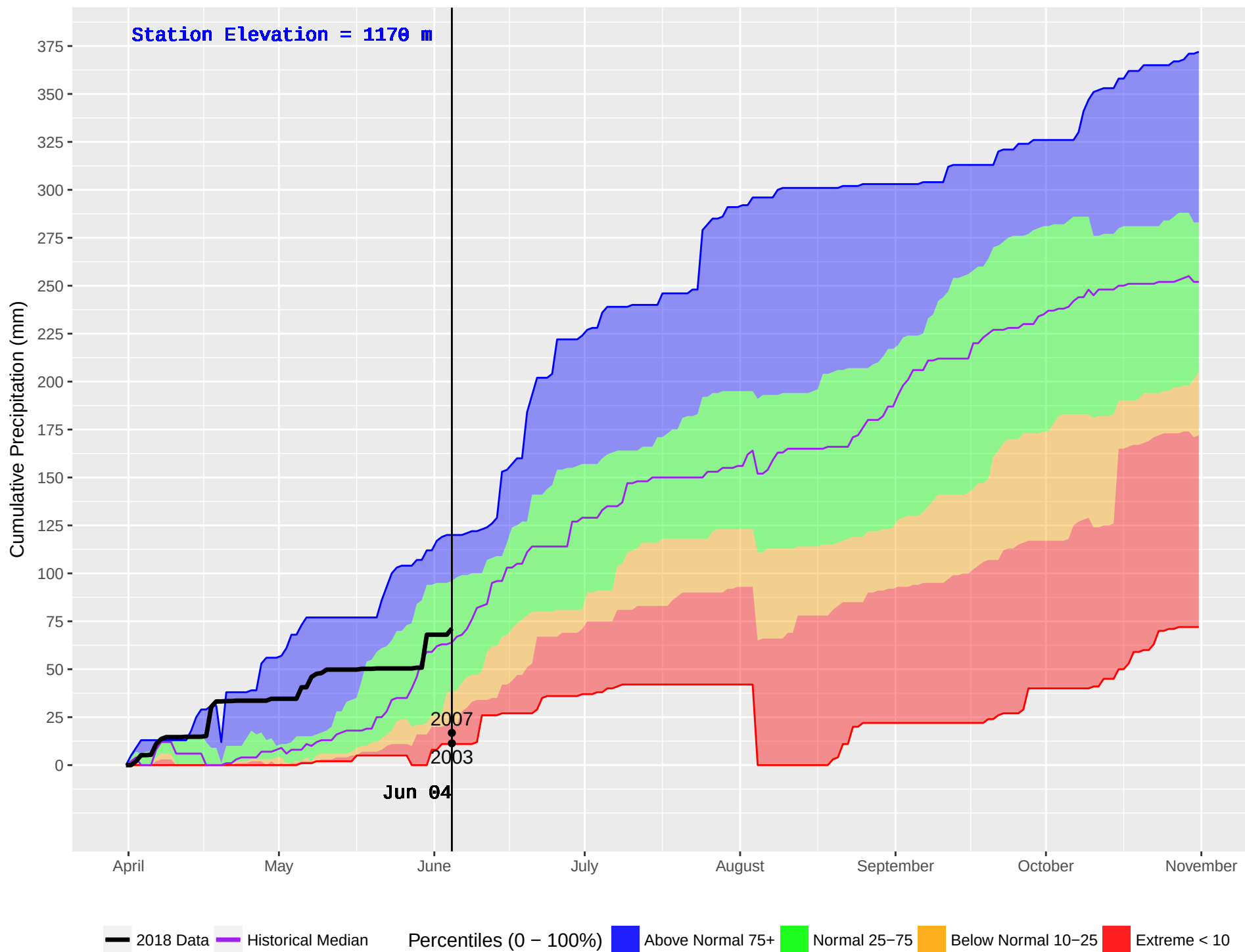
YOUNG LAKE (235) : Historical (2001–2016) and Current (2018) Noon Cumulative Precipitation
