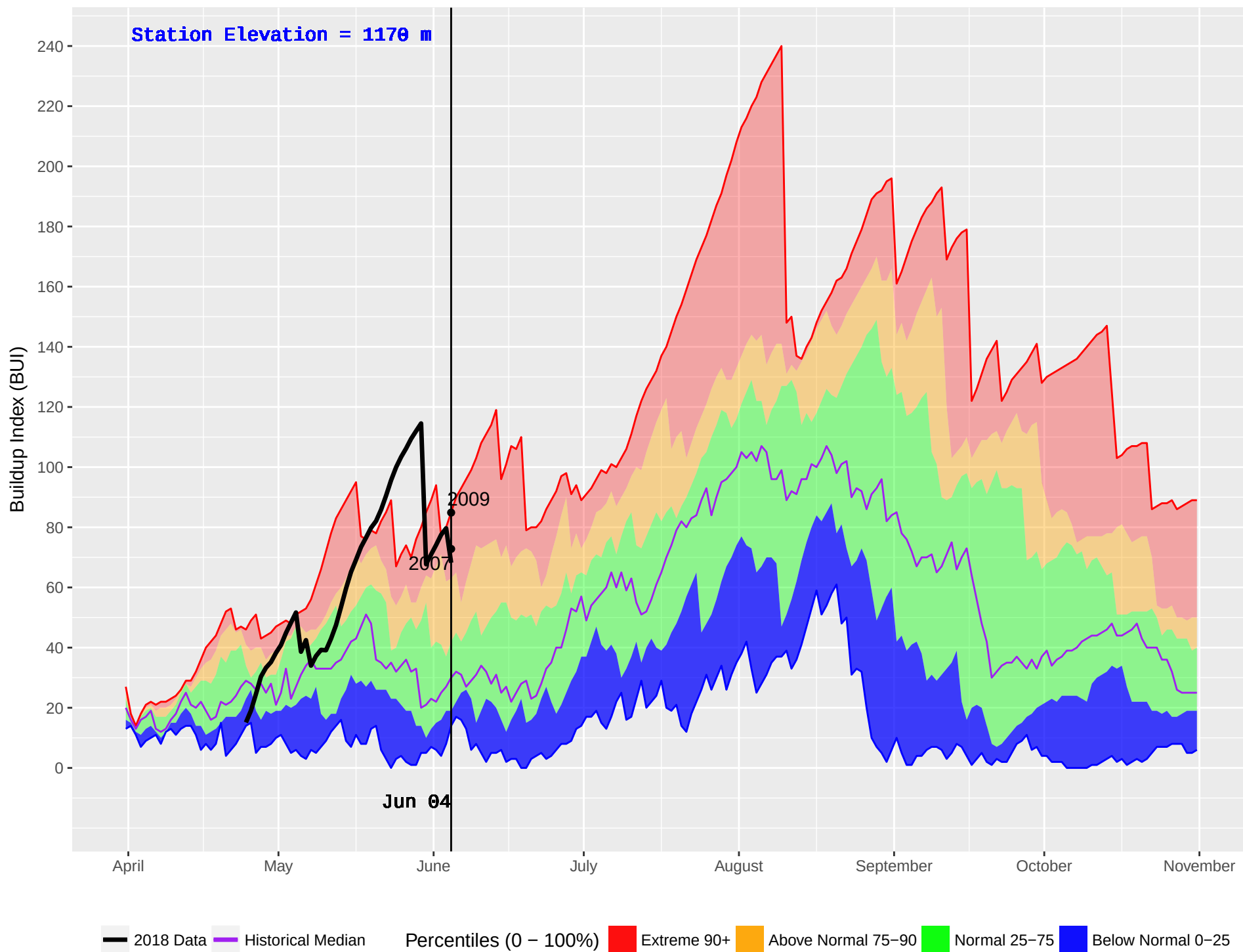
YOUNG LAKE (235) : Historical (2001–2016) and Current (2018) Noon Buildup Index (BUI)
