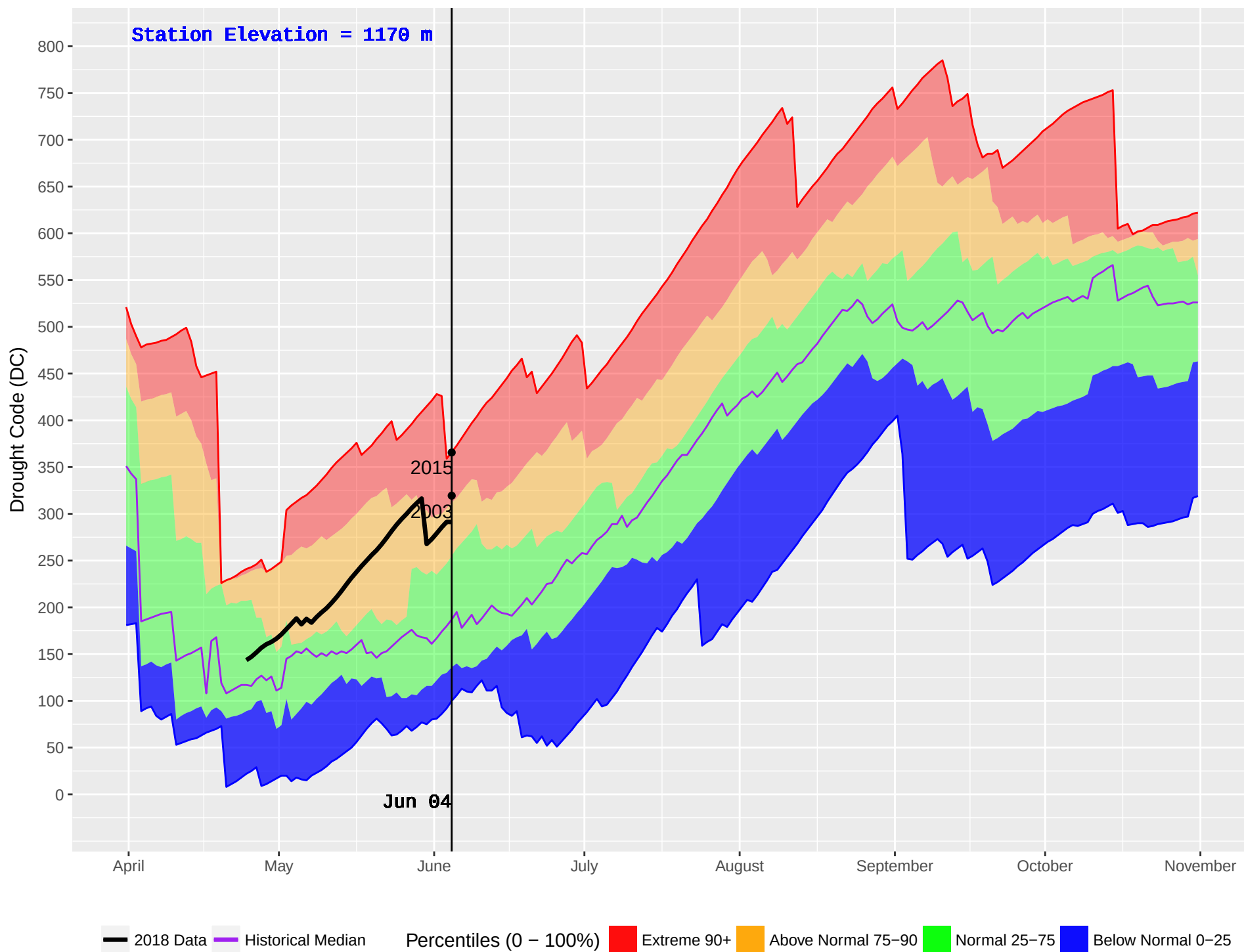
YOUNG LAKE (235) : Historical (2001–2016) and Current (2018) Noon Drought Code (DC)
